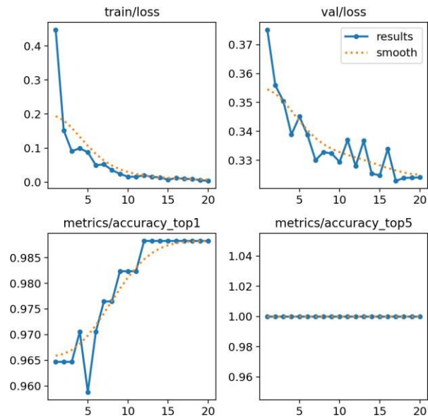
Figure 5. Training and Validation of Accuracy and Loss for YOLO-v8
