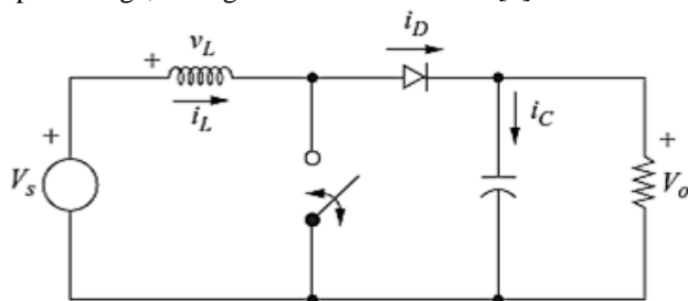
Figure 2: Basic circuit of a DC-to-DC Boost Converter [5]
