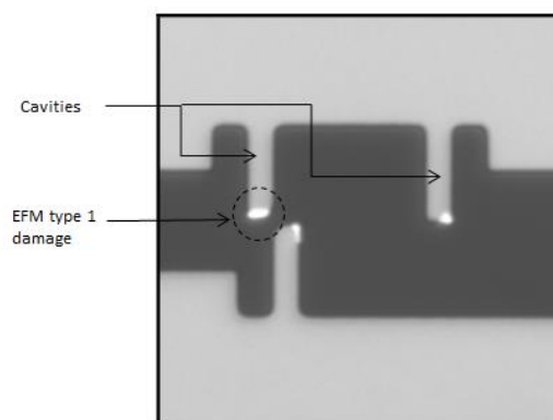
Figure 2: EFM type 1 damaged are seen at bottom corner cavities after reticle test plate inside monopod was expose to ambient electric field. Image was taken with optical microscope [8].
