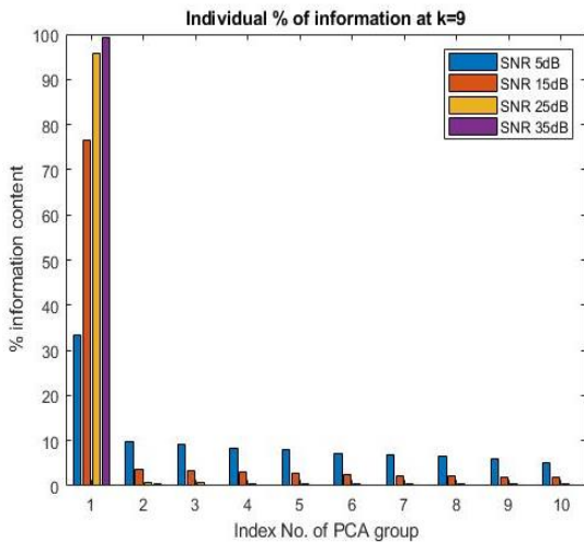
Figure 8: Individual information (%) corresponding to 10 principal components over Rician channel at k=9
