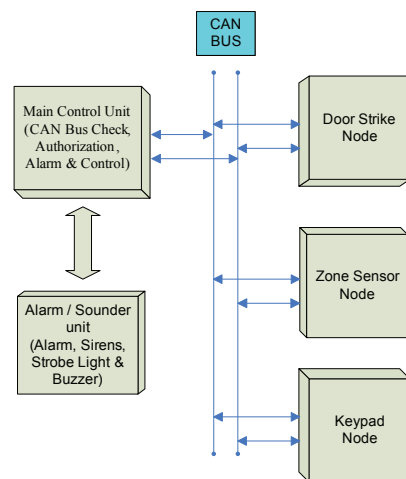
Figure 3: Security System block Diagram
