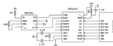
Figure 2: CAN controller and CAN Transceiver Connection
