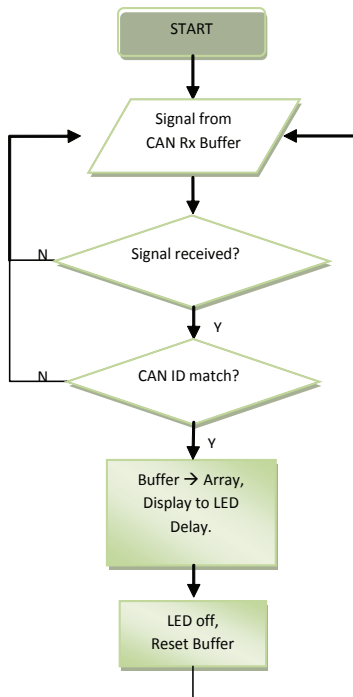
Figure 6: Example Flowchart of the Receiver Program.
