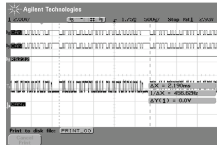
Figure 7: MSO output of CAN activity.
