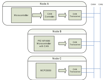
Figure 1: General Block Diagram of CAN bus system
