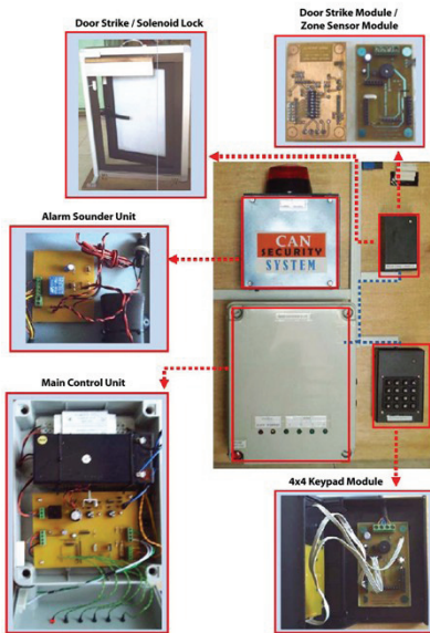
Figure 4: Security System Using CAN bus
