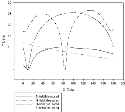
Figure 8: Measured and simulated radiation pattern at 2.4GHz (Design I).
