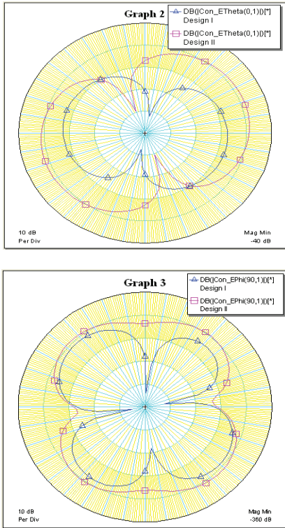
Figure 5: The radiation pattern for Design I and Design II at frequency 2.4GHz.
