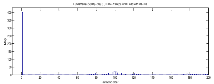
Figure 11: THD_v for IRVMLI with M_a=1.0 .
