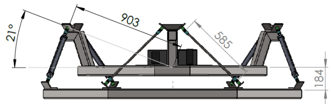
Figure 7: Home Position of the Platform Simulator
