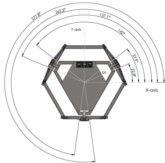
Figure 6: Position of Centroid of the Moving Platform (the End Effector) Among the Upper Universal Joints
