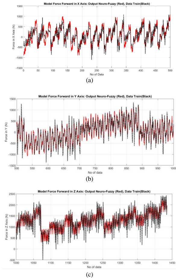
Figure 8: Generating data of Total Force compared with the Neuro-Fuzzy Model in Axis X (a), Axis Y (b) and Axis Z(c)
