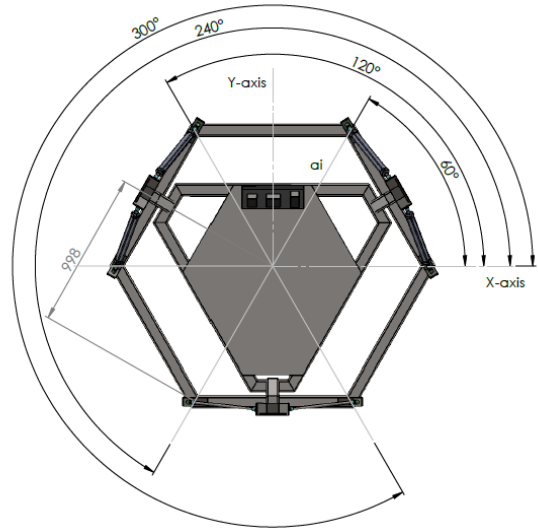
Figure 5: Position of Centroid of the Fix Platform Among the Lower Universal Joints
