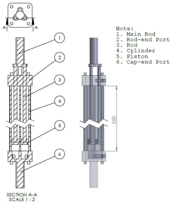
Figure 1: Multi Piston Pneumatic Actuator
