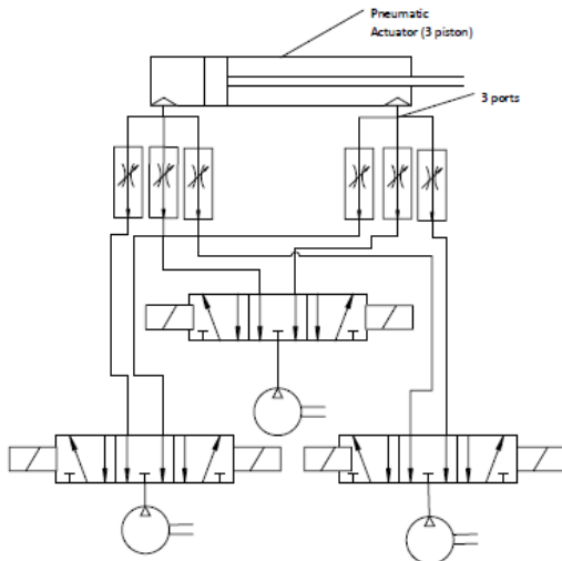
Figure 4: The Pneumatic Circuit Diagram
