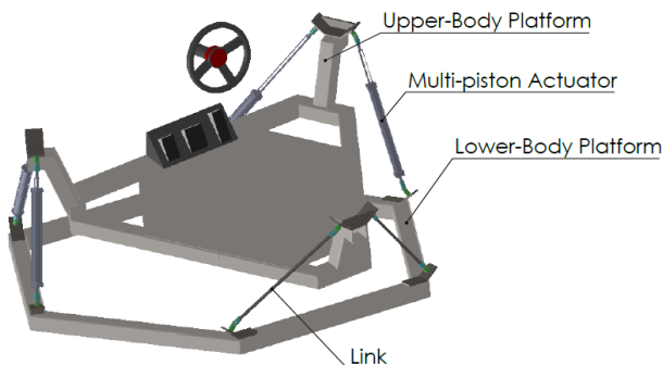
Figure 2: Three Dimension Platform Simulator
