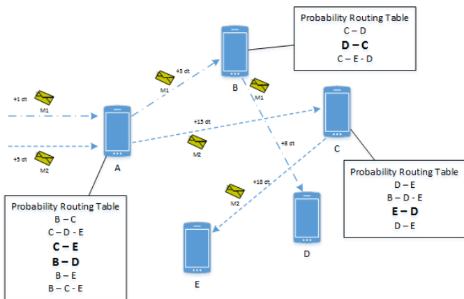
Figure 6: Message relay vector using Hybrid PRoPHET-EPIDEMIC
