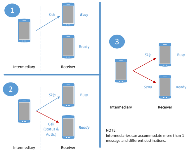
Figure 5: Stages of message relay from an intermediary device to a recipient
