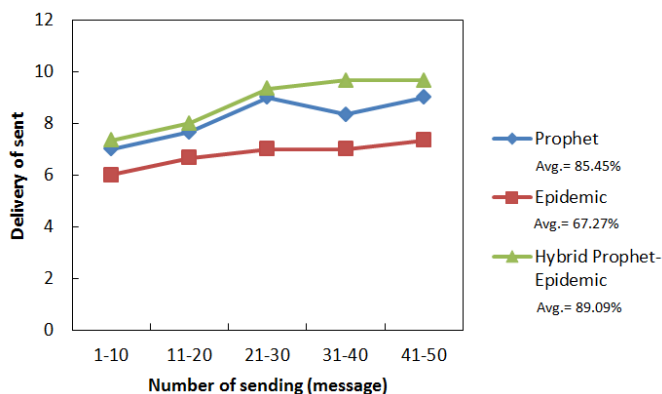
Figure 8: Comparison of success rate sending messages
