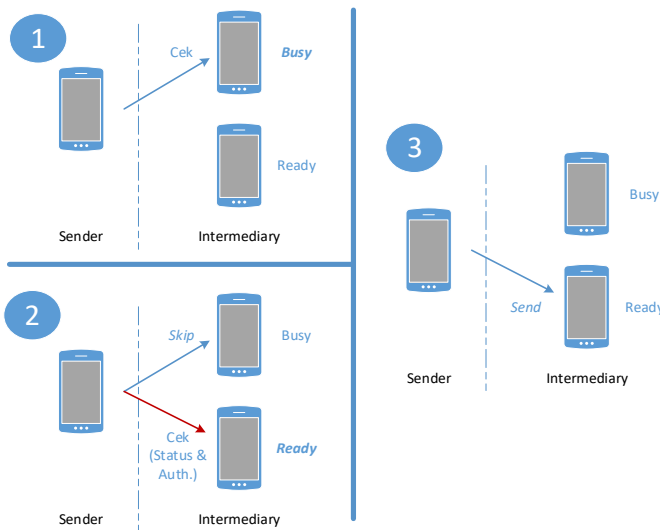
Figure 4: Stages of message relay from sender to intermediary device
