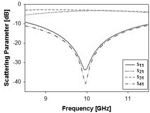
Figure 5: Scattering parameter performances for the proposed designed coupler
