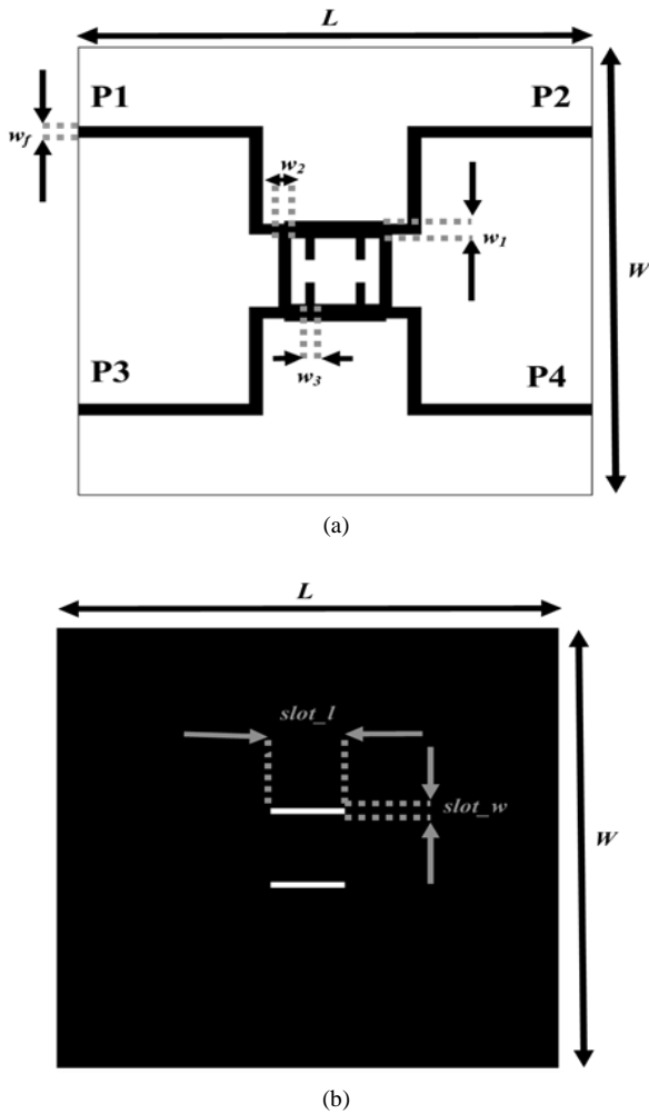
Figure 4: The proposed design of 5G coupler from the (a) top view (b) bottom view
