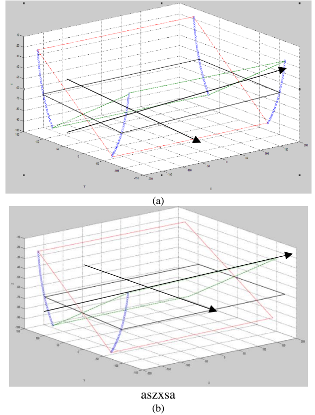
Figure 8: Positions of a_i^e for \theta_1 (Blackline – Initial position, Green Line – Ideal maximum platform position for Eversion, Red Line- Ideal Maximum platform position for Inversion)
