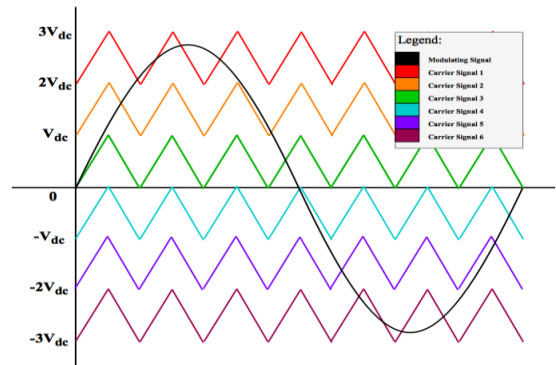
Figure 3: PD PWM with (m-1) Carrier Signal Waveforms
