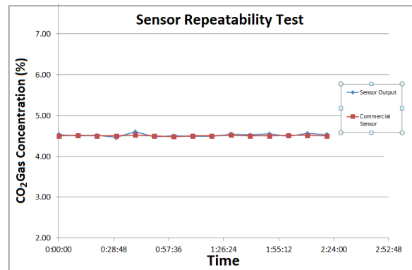
Figure 5: The results of developed optical fiber based gas sensor repeatability test.
