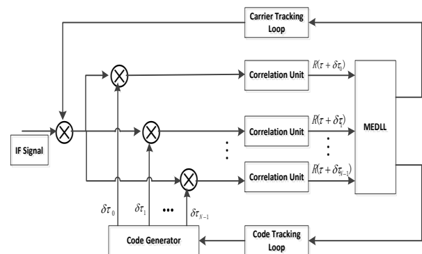
Figure 1: Block diagram of MEDLL
