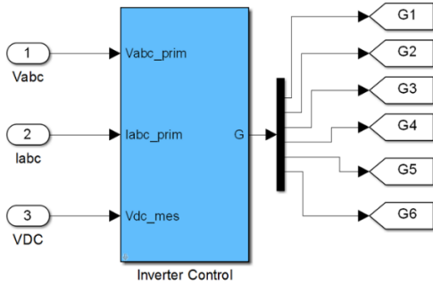
Figure 3: PWM controller block diagram
