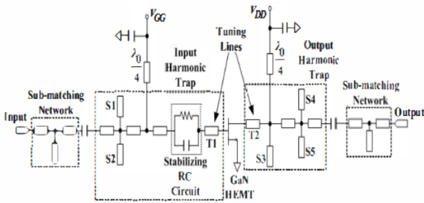
Figure 20: Schematic circuit of 2.0 GHz PA [38]
