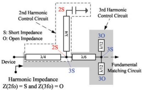
Figure 7: Proposed HCC of the class F PA [15]
