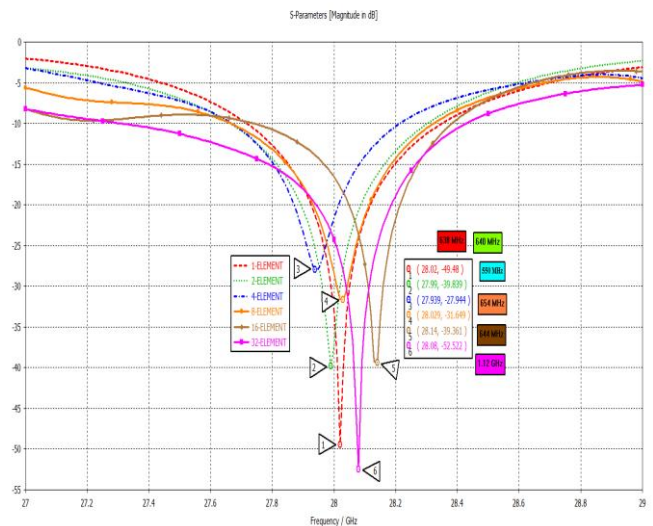
Figure 5: The Return loss for single patch until 32-Element patch array
