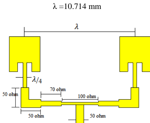
Figure 2: The front view of 2x1 patch antenna
