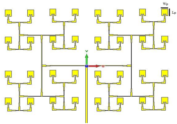
Figure 4 The front view of 4x8 patch array antenna
