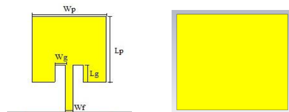
Figure 1: The front view of and back view of single patch antenna
