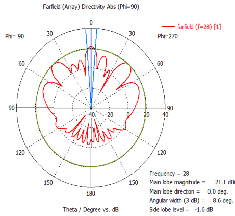
Figure 7: The Directivity (polar) for 32-Element patch array antenna
