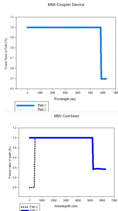
Figure 7: MMI-Coupler and MMI-Combiner power ratio in path
