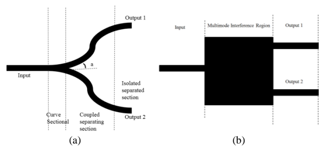
Figure 1: (a) Y-coupler diagram, (b) MMI-coupler diagram
