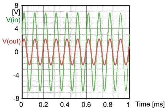
Figure 3: Transient analysis of Wien Bridge Oscillator
