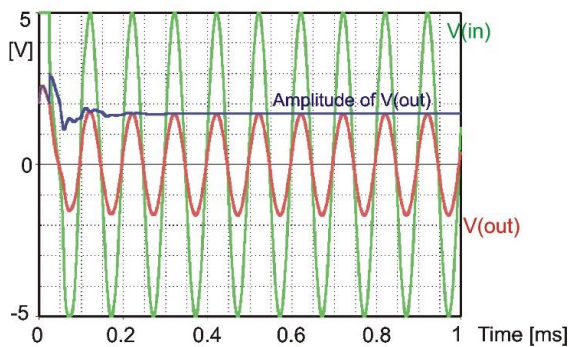
Figure 5: Transient analysis of Wien Bridge Oscillator with AGC
