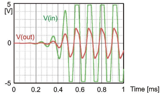
Figure 4: Transient analysis of Wien Bridge Oscillator with operational amplifier
