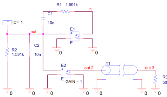
Figure 7: Wien Bridge Oscillator with AGC
