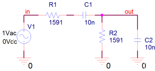
Figure 2: Wien Bridge
