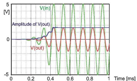
Figure 6: Transient analysis of Wien Bridge Oscillator with AGC
