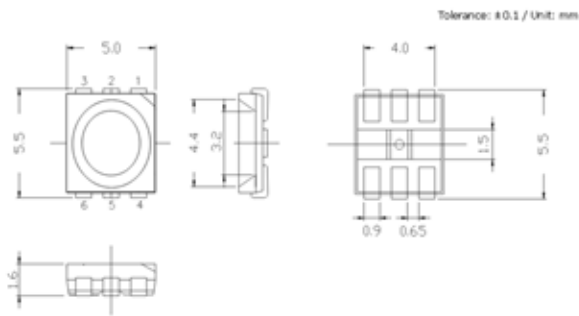
Figure 1: structure of the SMD5050 LED
